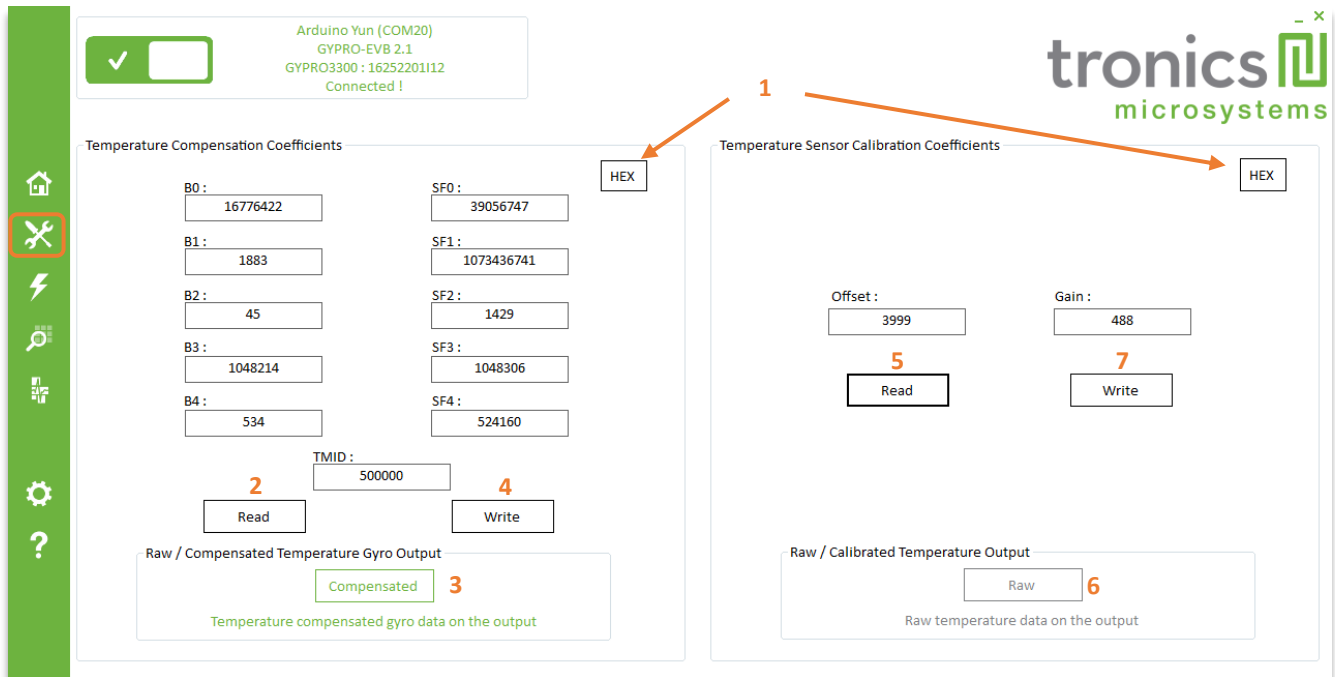
Figure 5: Tronic's Evaluation Tool - "System Register (SR)" tab
