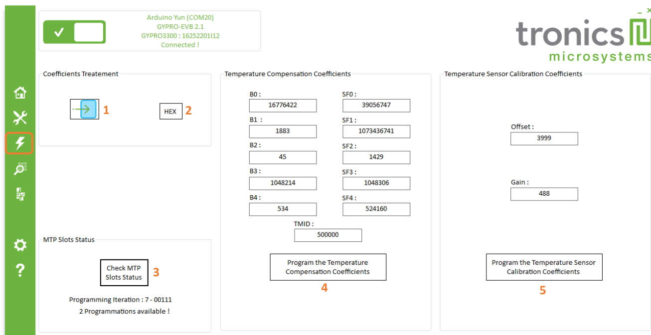
Figure 6 : Tronic's Evaluation Tool – “Multi-Time-Programmable (MTP)” tab
